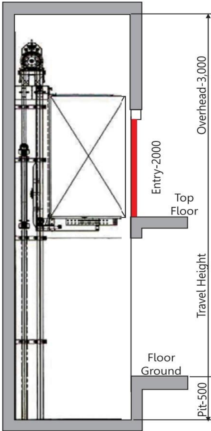
HOISTWAY ELEVATION DRAWING
